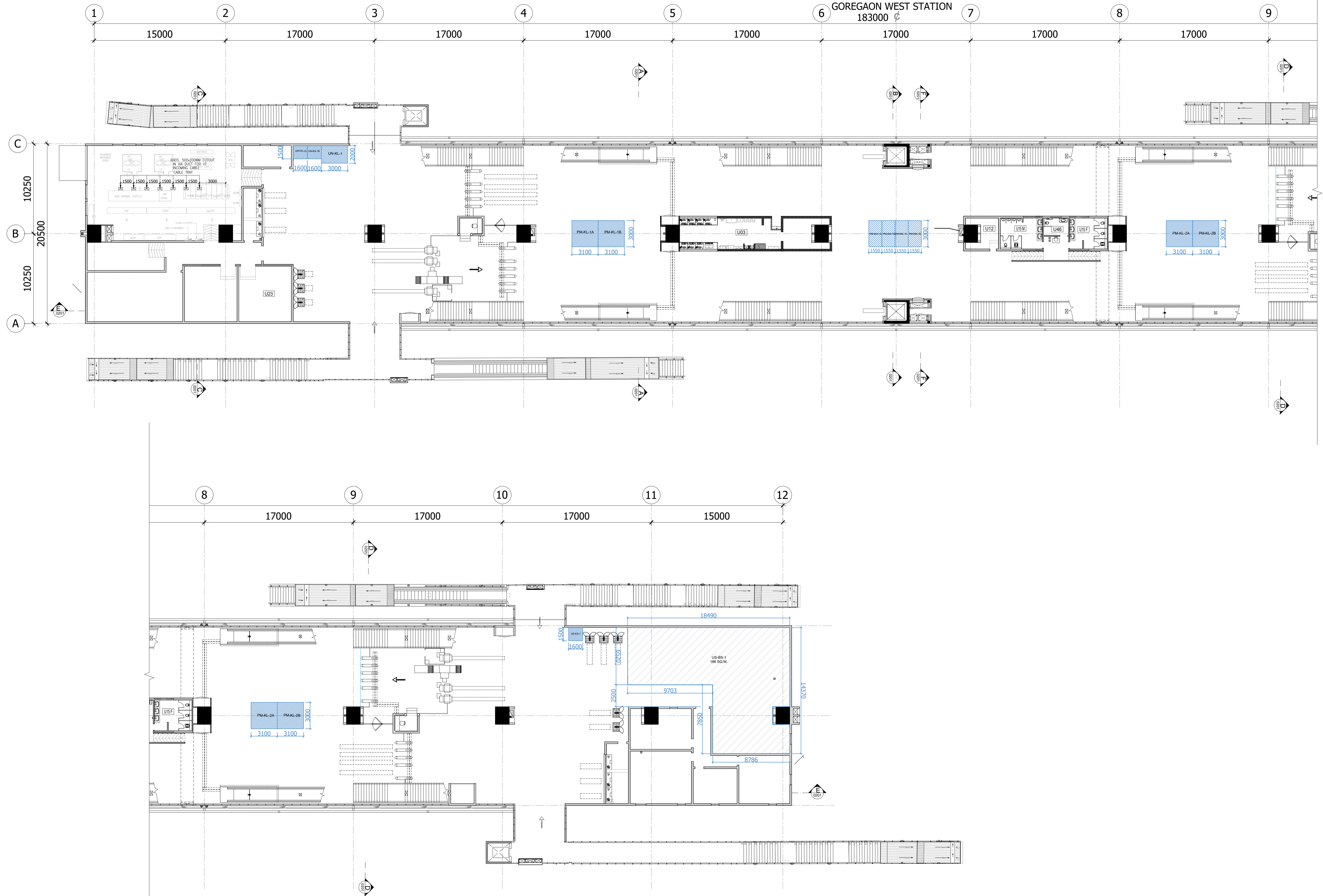
GOREGAON WEST METRO STATION- CONCOURSE LEVEL PLAN
