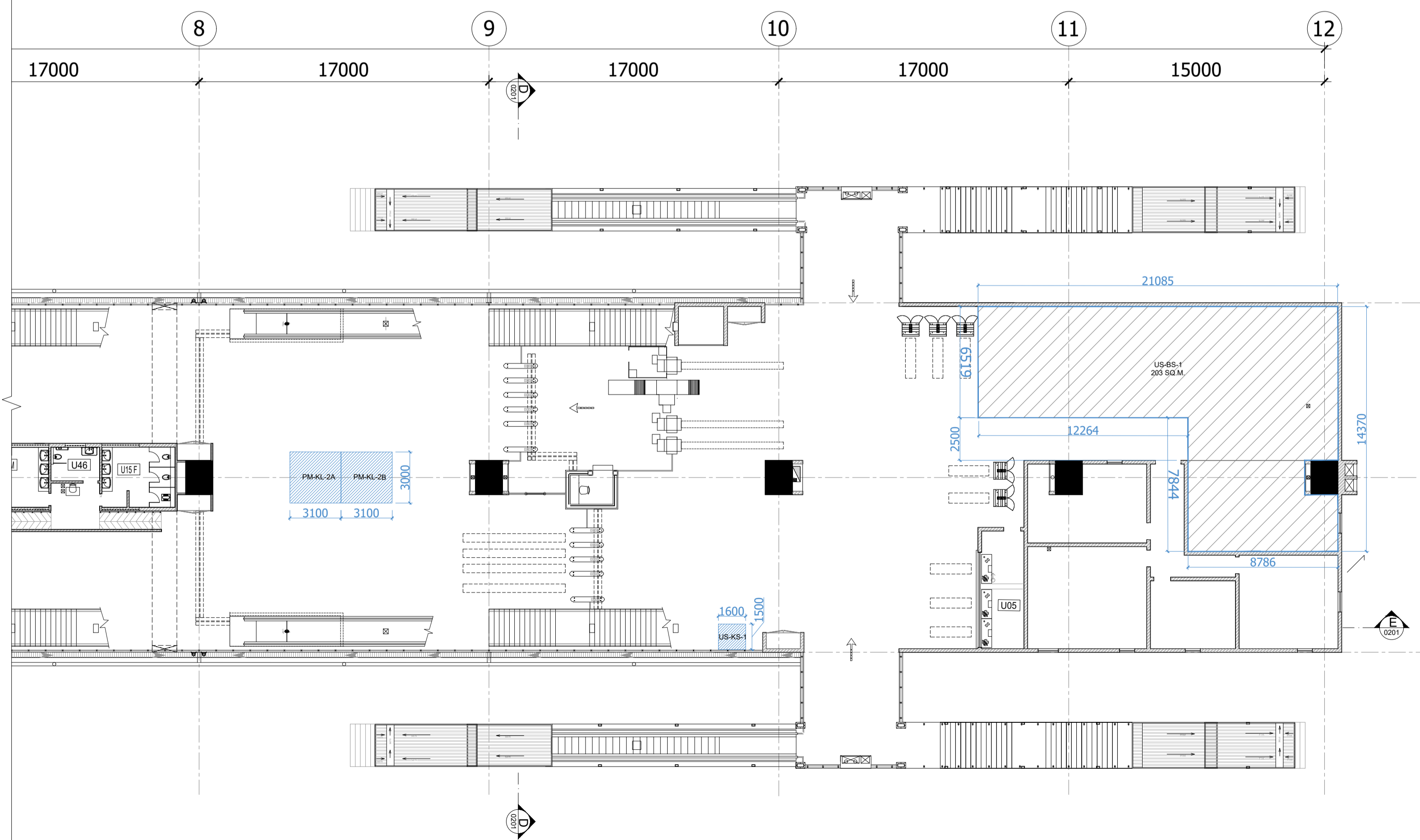
LOWER MALAD METRO STATION- CONCOURSE LEVEL PLAN
