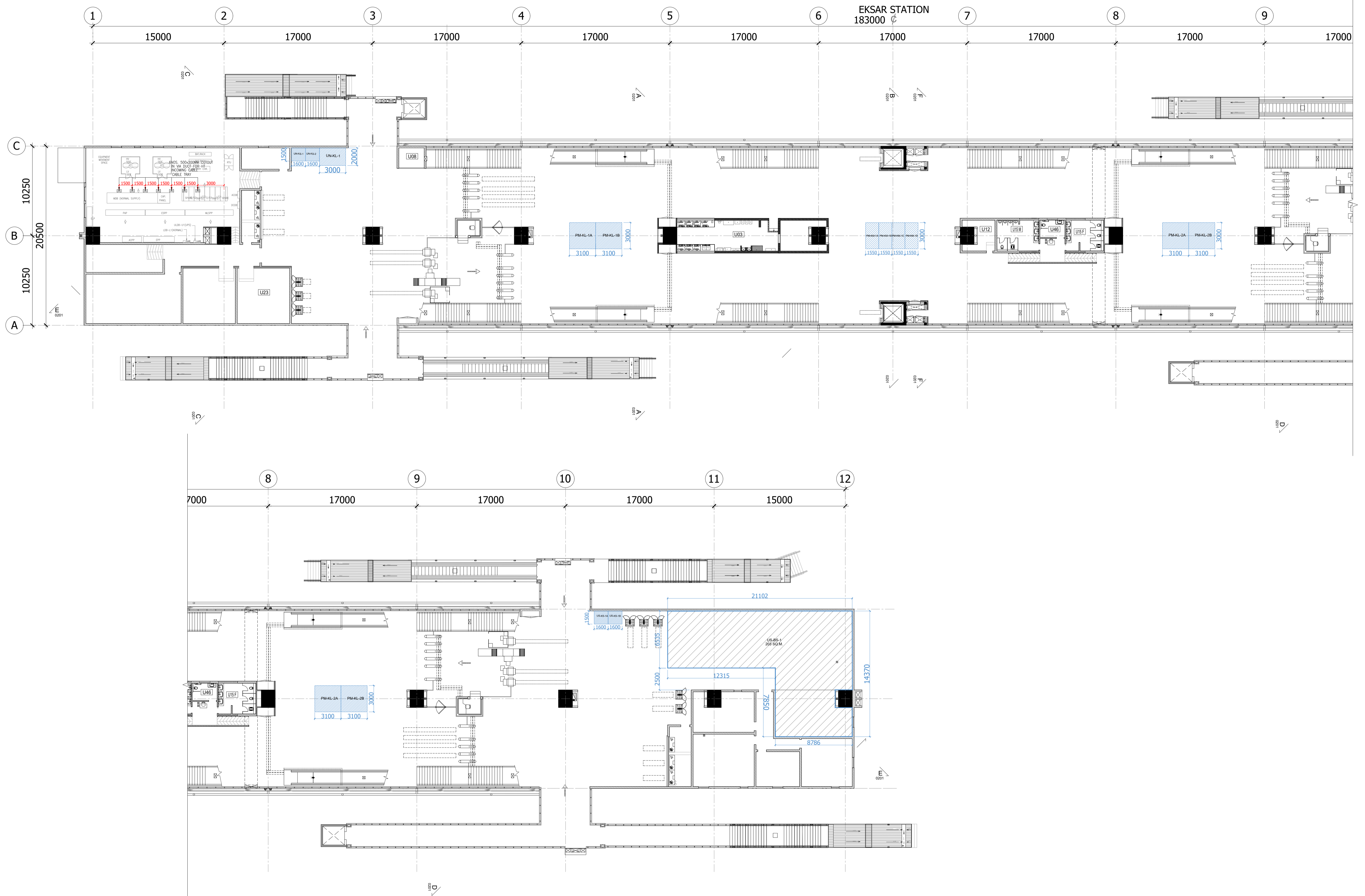
EKSAR METRO STATION- CONCOURSE LEVEL PLAN
