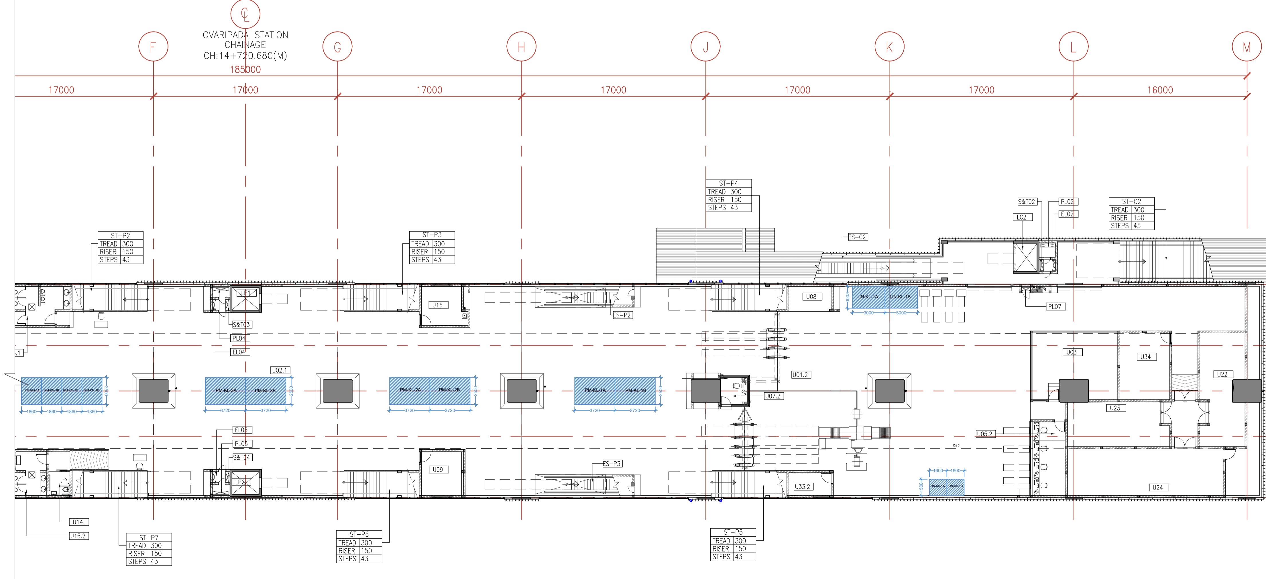
OVARIPADA METRO STATION- CONCOURSE LEVEL
