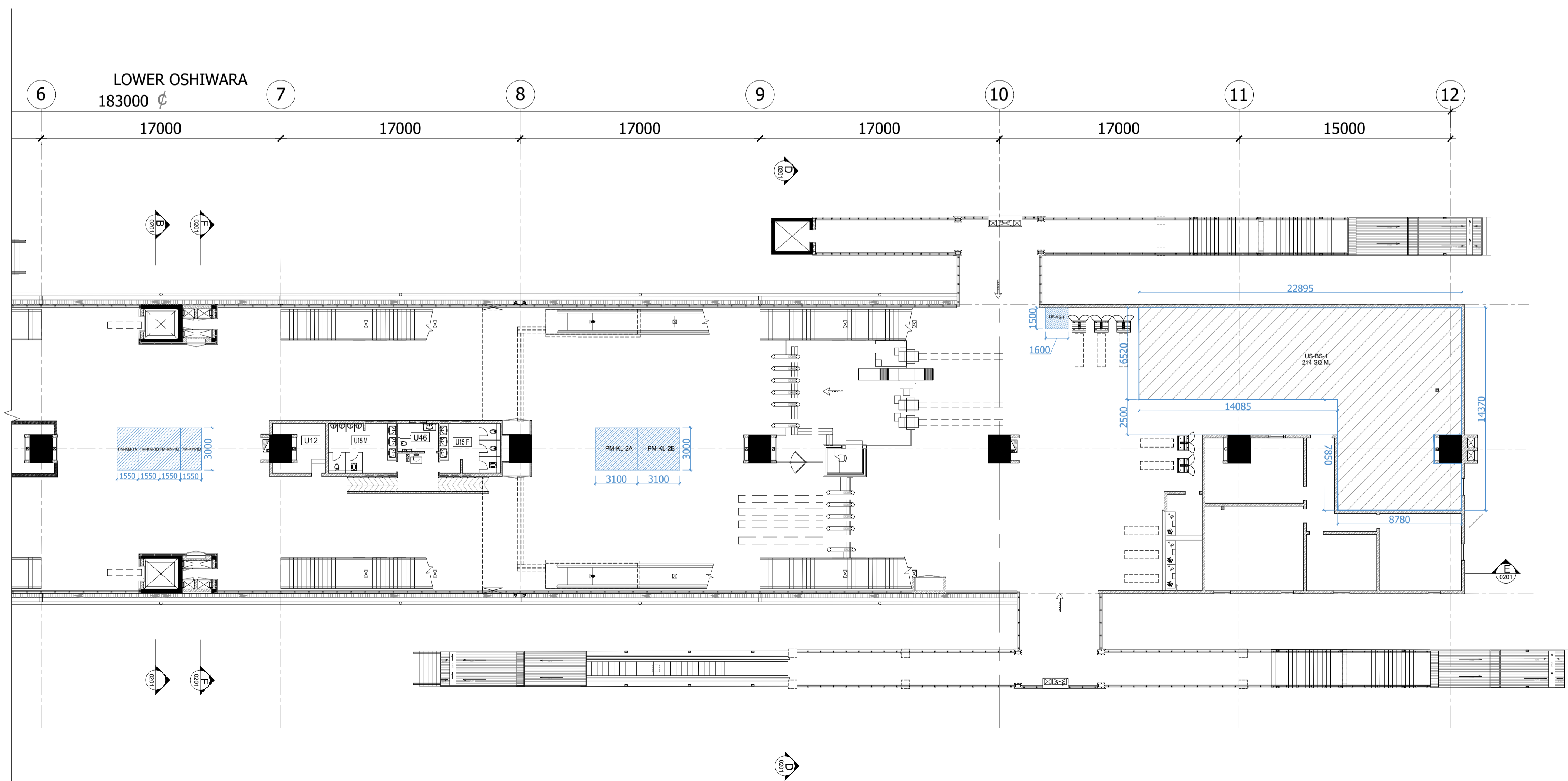
LOWER OSHIWARA METRO STATION- CONCOURSE LEVEL PLAN
