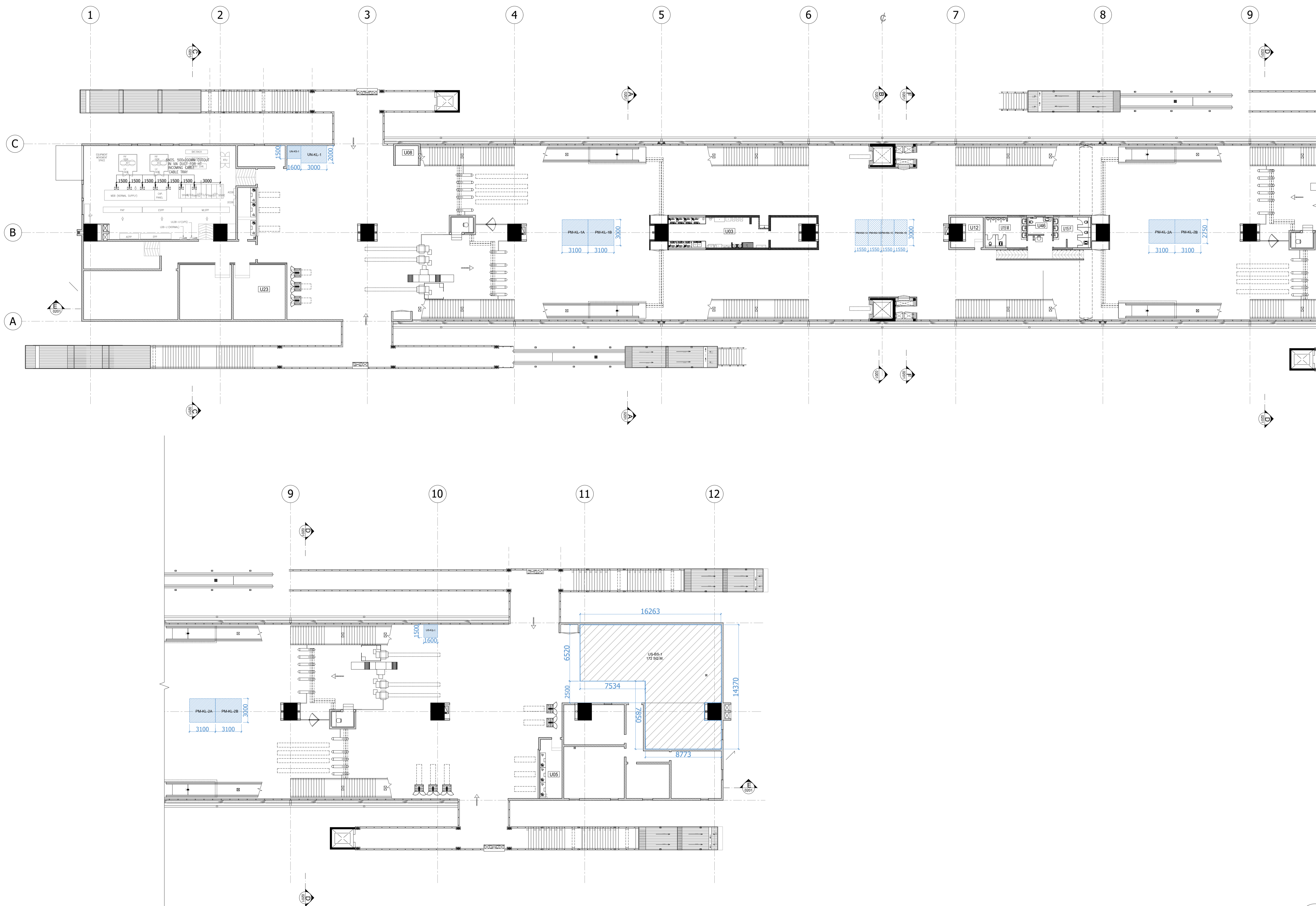
PAHADI EKSAR METRO STATION- CONCOURSE LEVEL PLAN
