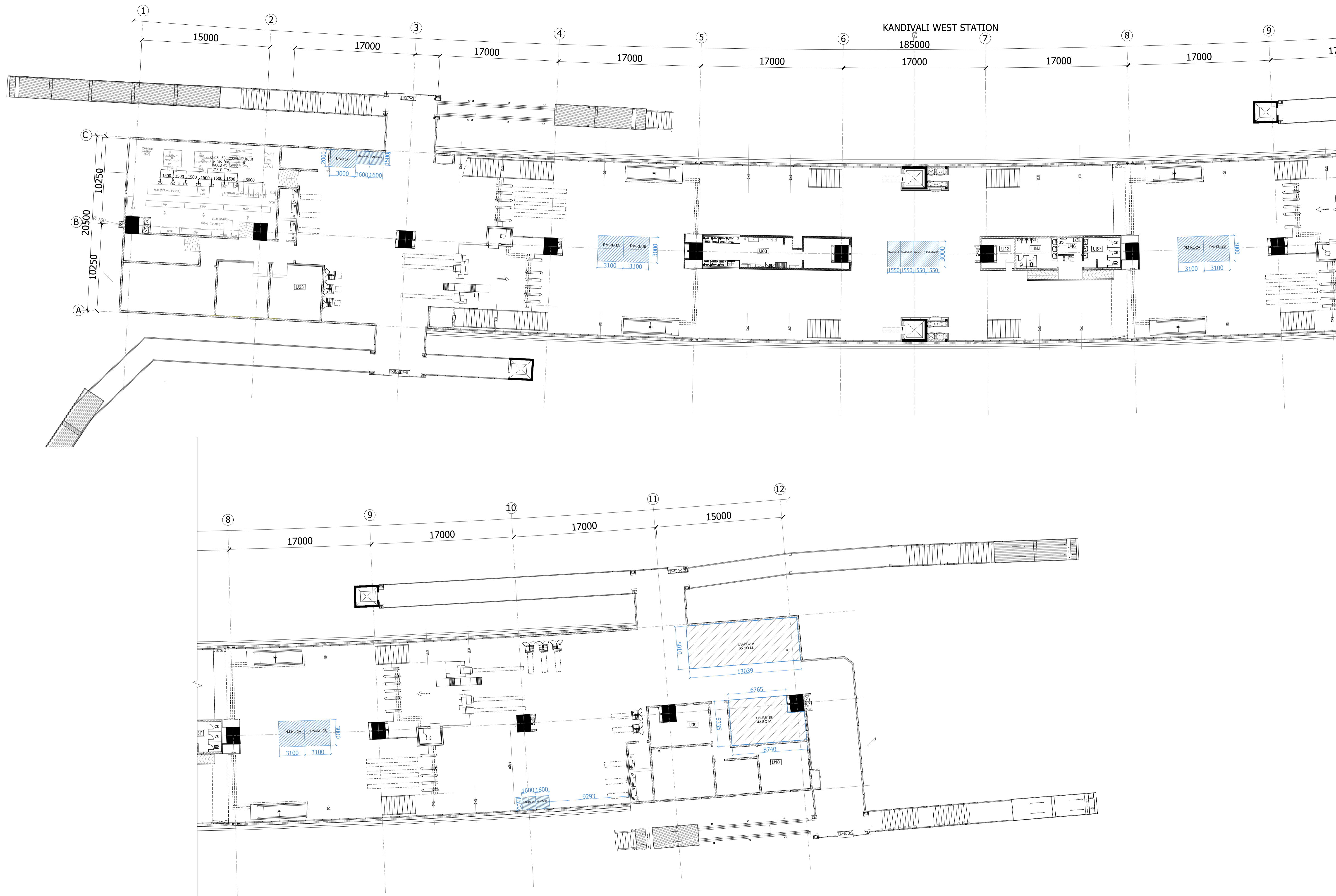
KANDIVALI WEST METRO STATION- CONCOURSE LEVEL PLAN
