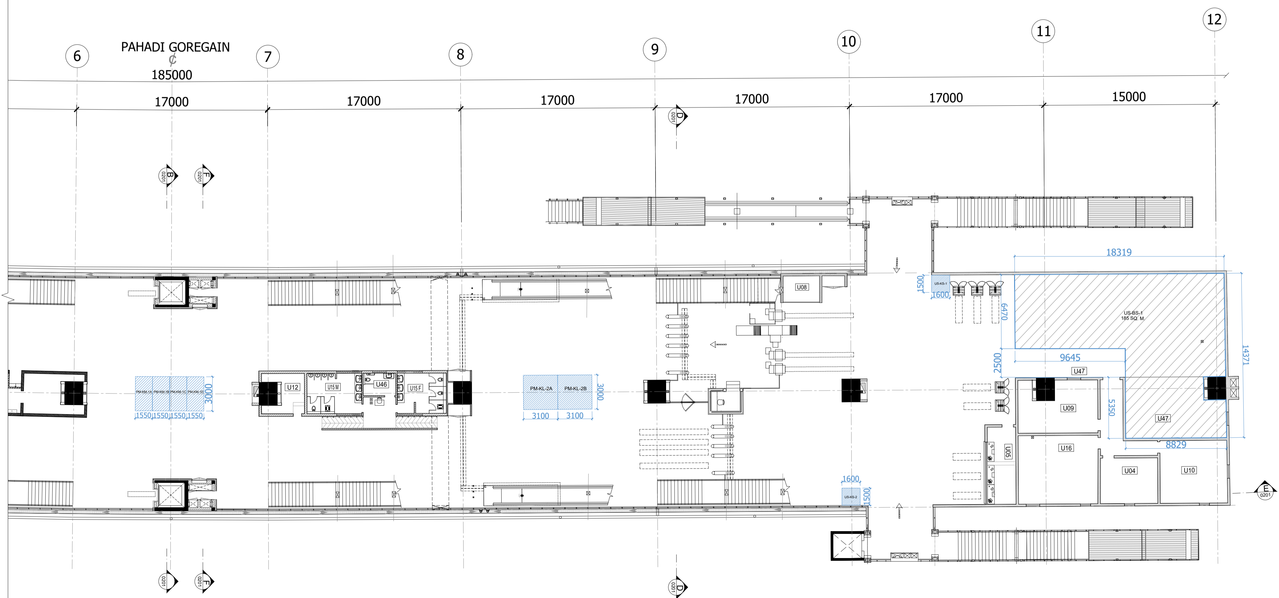
PAHADI GOREGAON METRO STATION- CONCOURSE LEVEL PLAN
