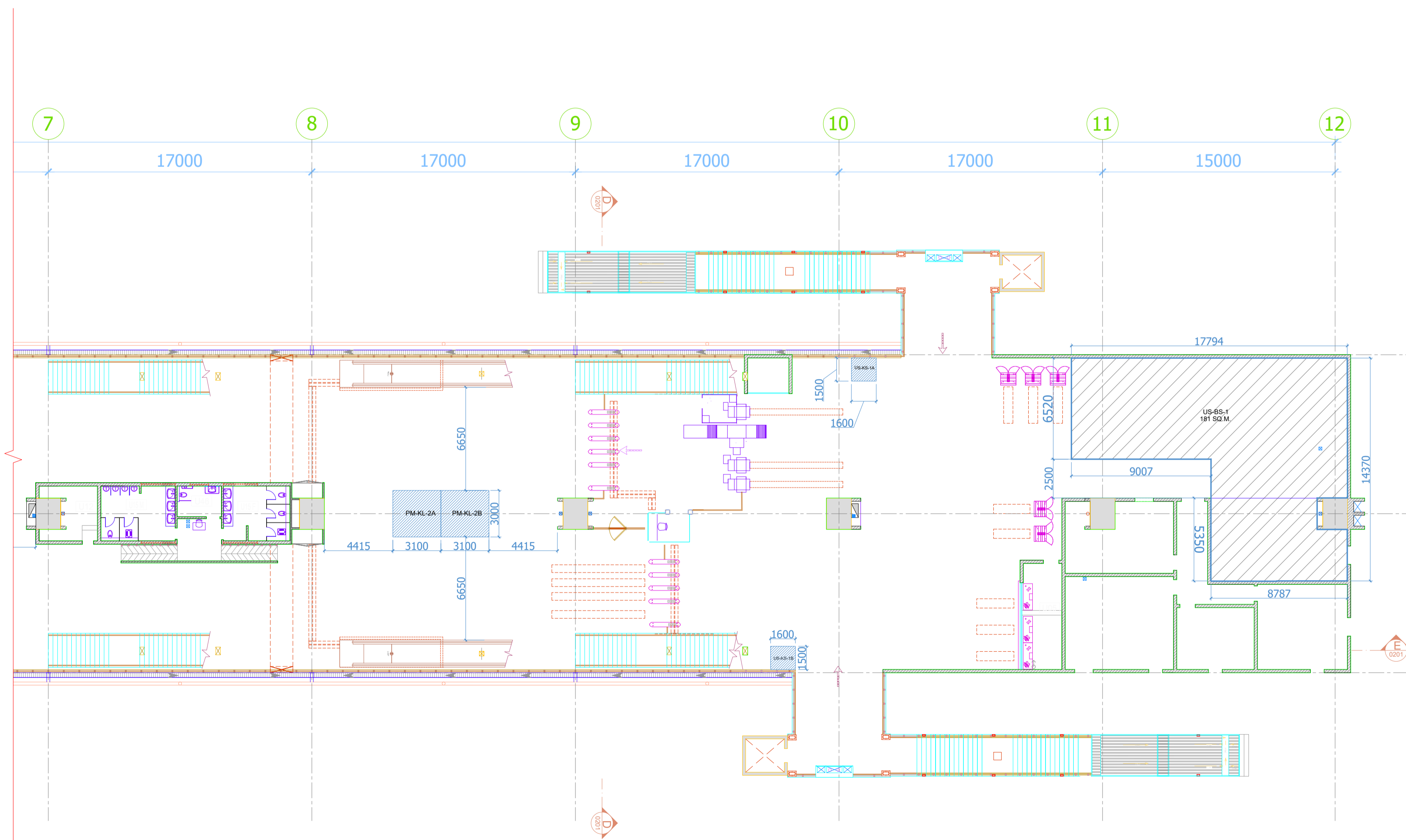
MALAD WEST METRO STATION- CONCOURSE LEVEL PLAN
