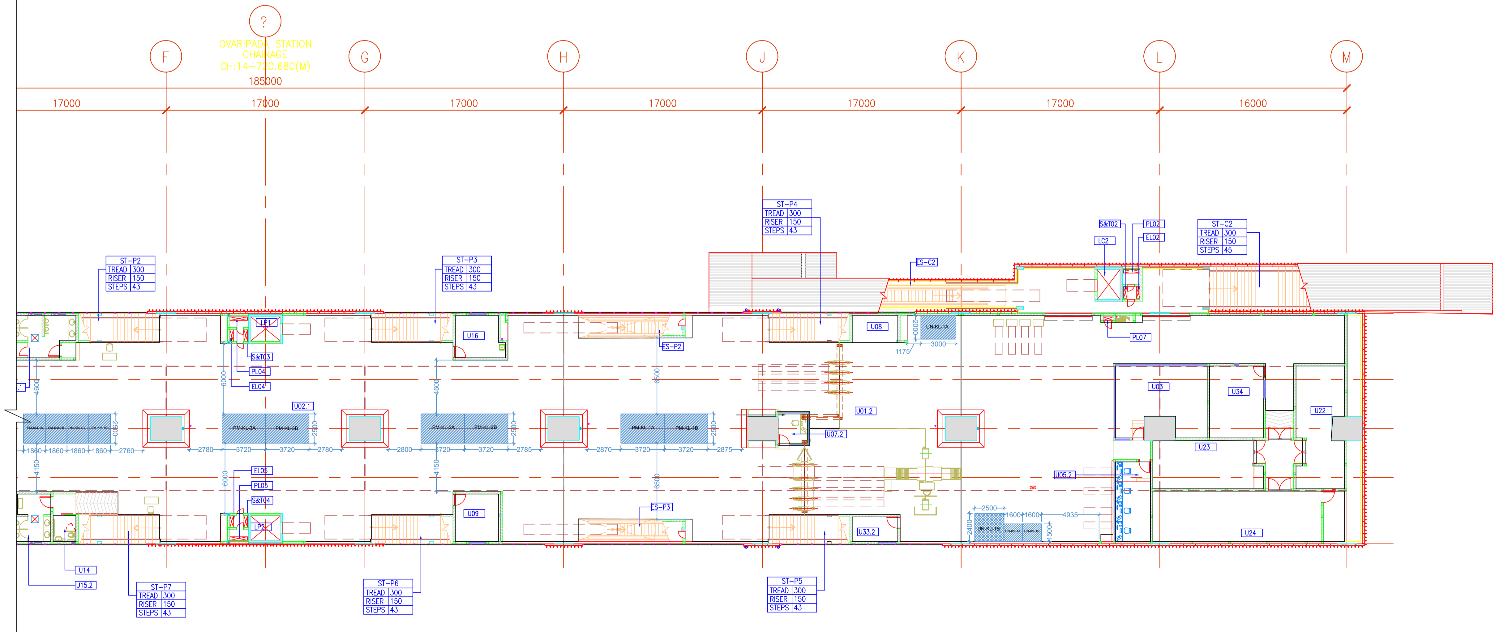
OVARIPADA METRO STATION- CONCOURSE LEVEL
