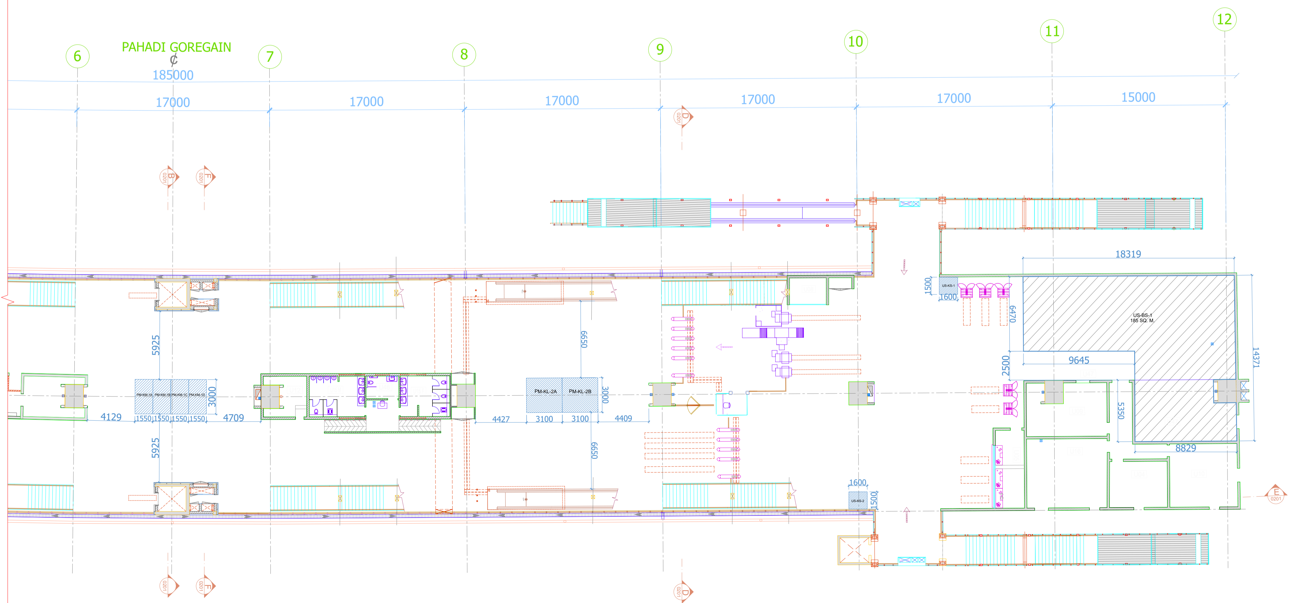
BANGUR NAGAR METRO STATION- CONCOURSE LEVEL PLAN
