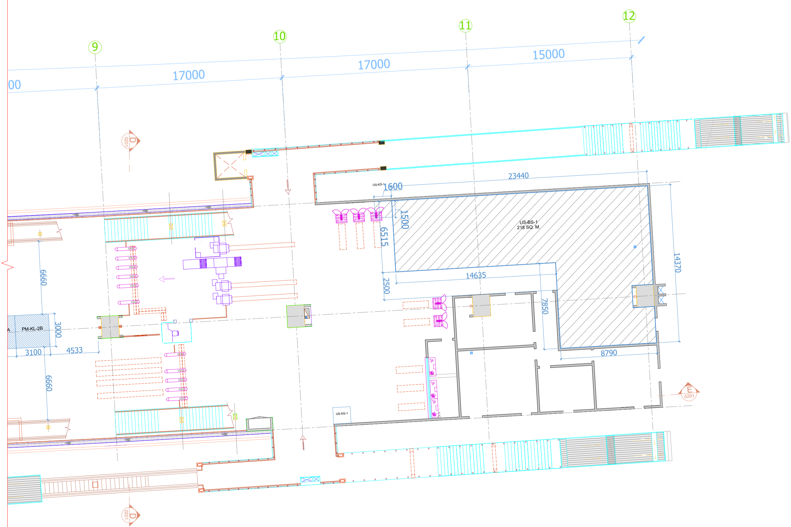
BORIWALI WEST METRO STATION- CONCOURSE LEVEL PLAN
