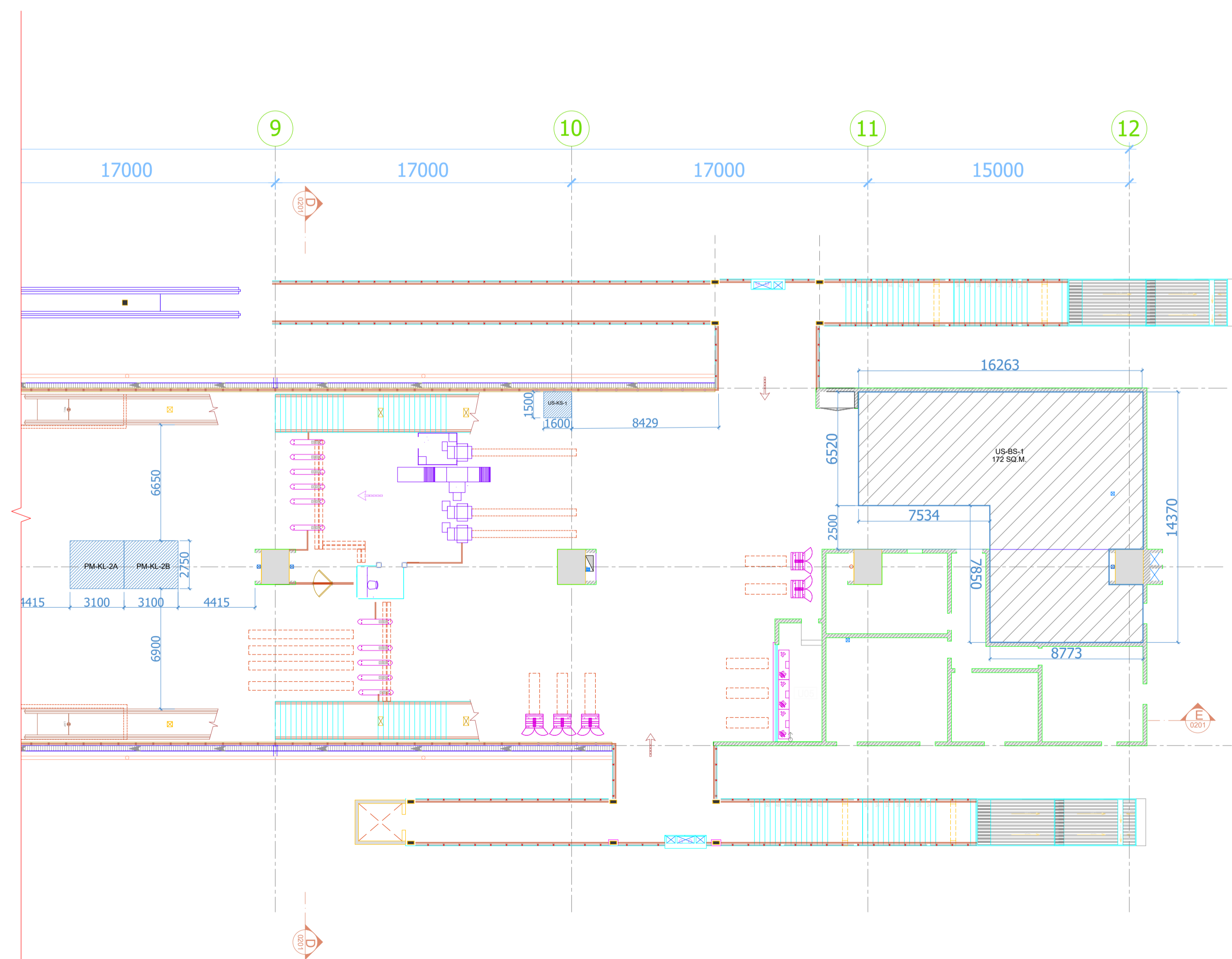
SHIMPOLI METRO STATION- CONCOURSE LEVEL PLAN
