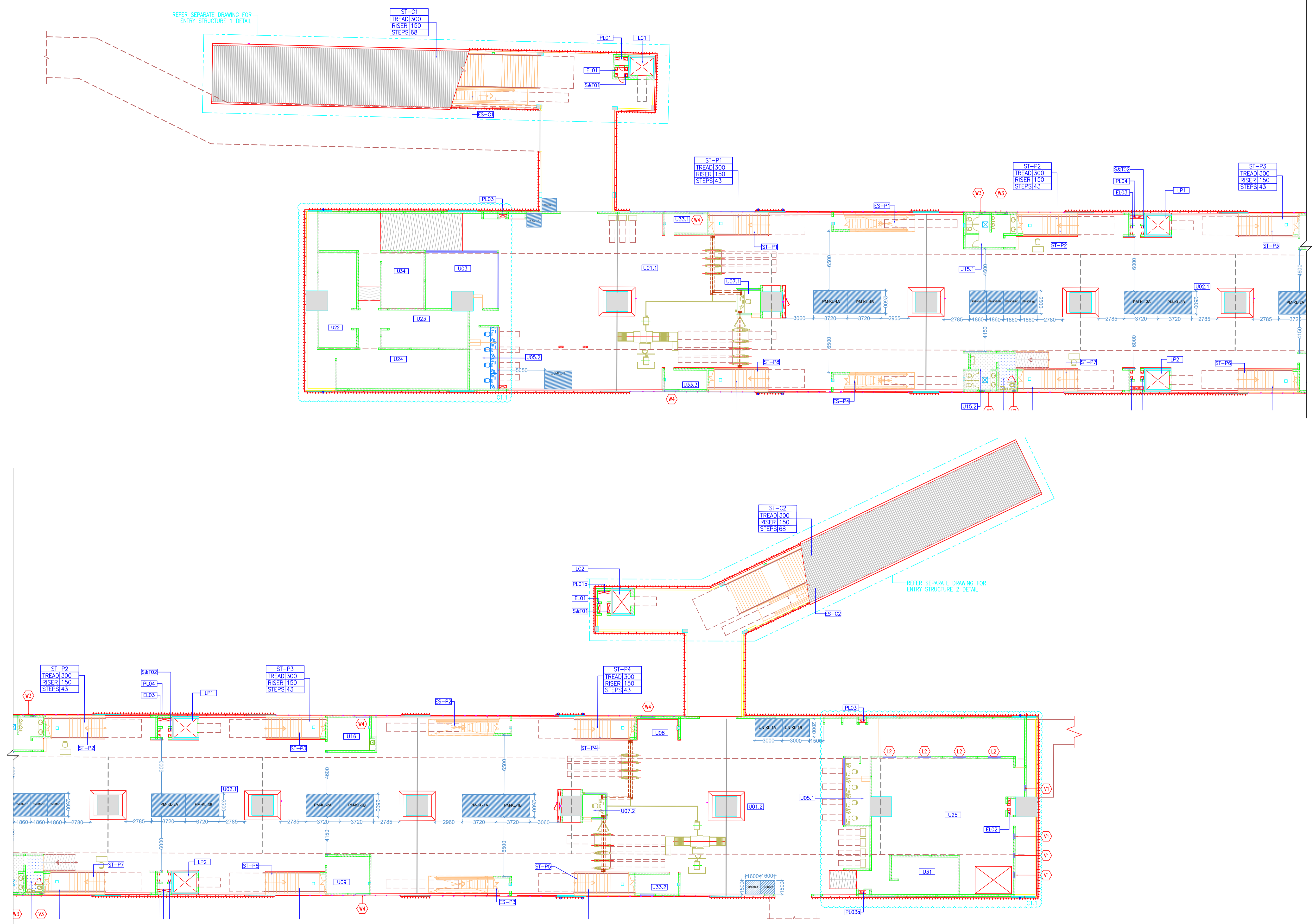
GOREGAON EAST METRO STATION- CONCOURSE LEVEL
